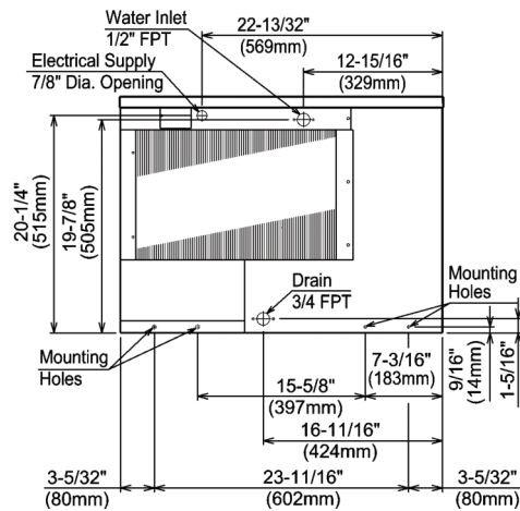
AIR-COOLED UNIT
